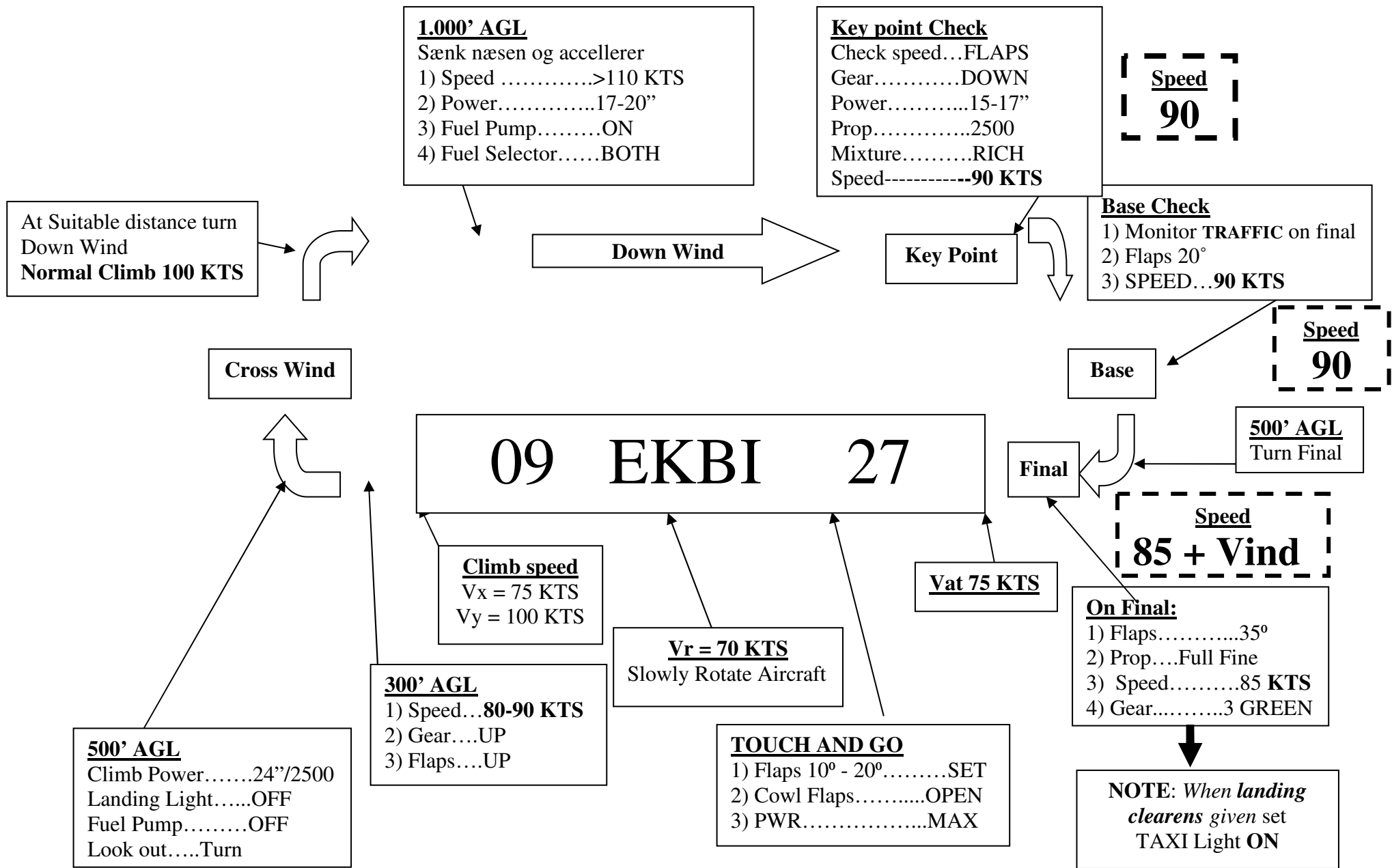
Landingsrunde profil for Commander 114B
