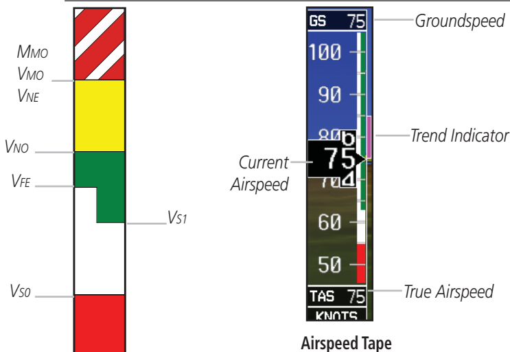
Typical Airspeed Tape Markings
